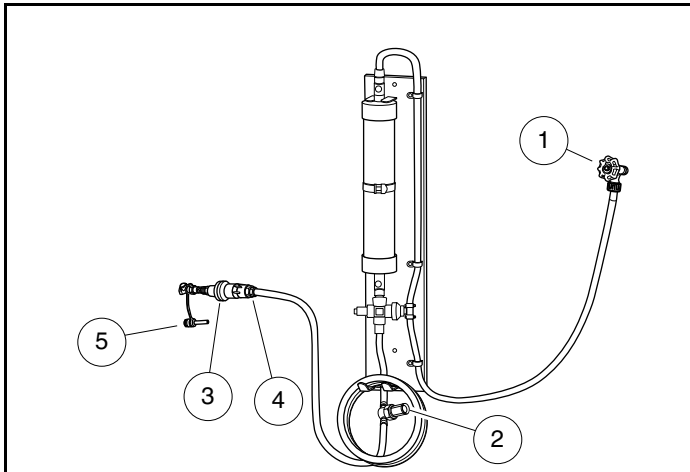
Figure 25 Connecting Hose with Filter to Water Source
