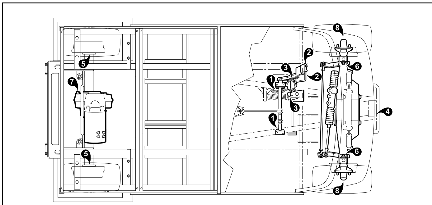
2777 Figure 22 Lubrication Points – Electric Vehicles
