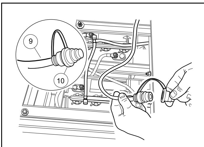
Figure 27 Dust Cap
