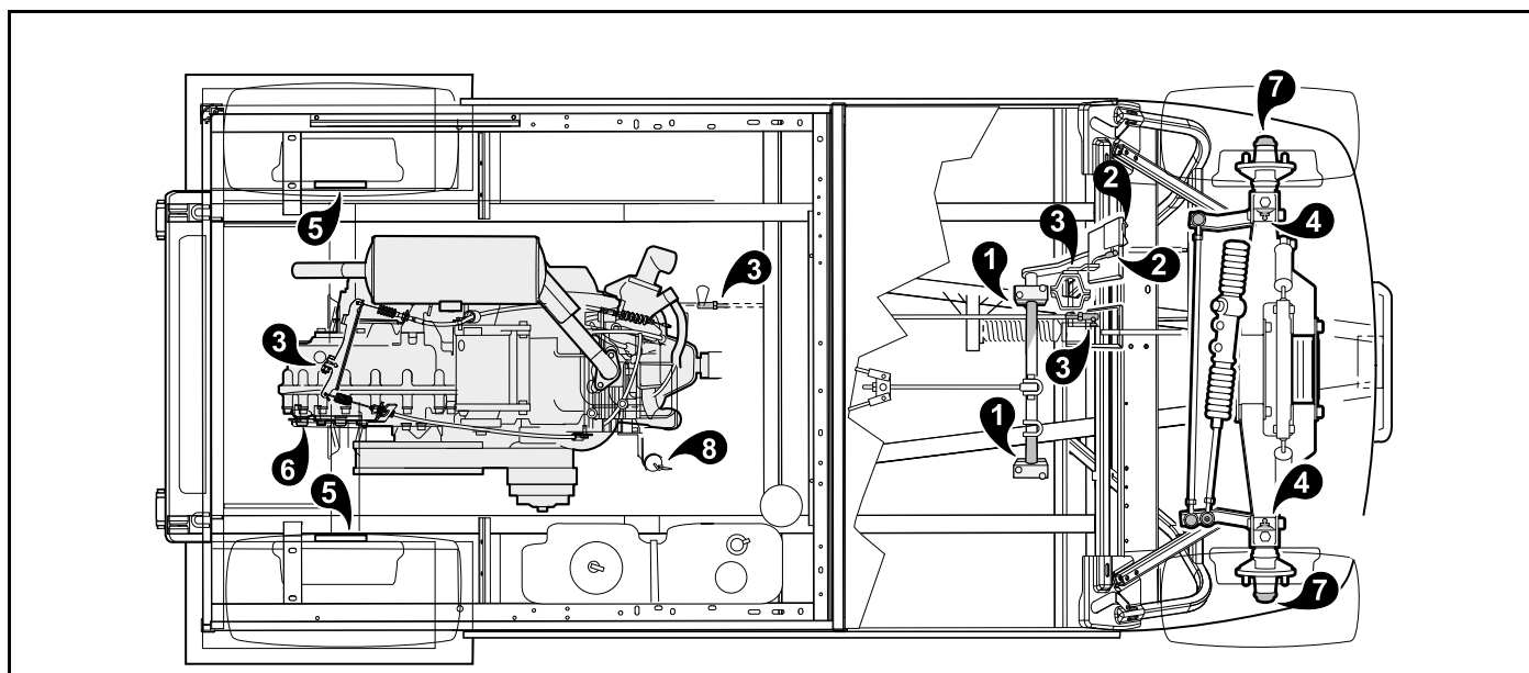
Figure 23 Lubrication Points – Gasoline Vehicles
