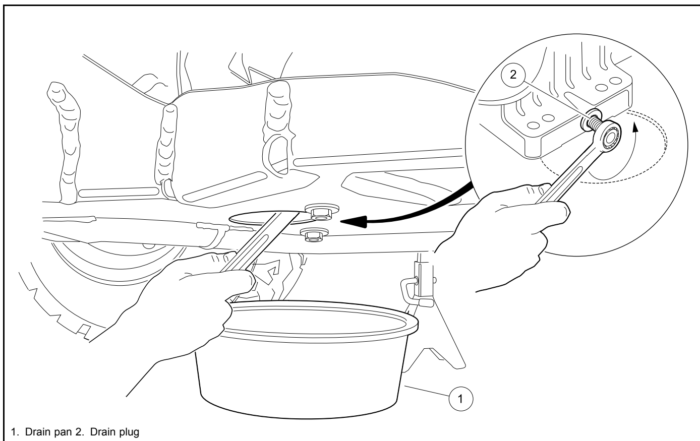
2667 Figure 37 Engine Oil Drain Plug and Pan
