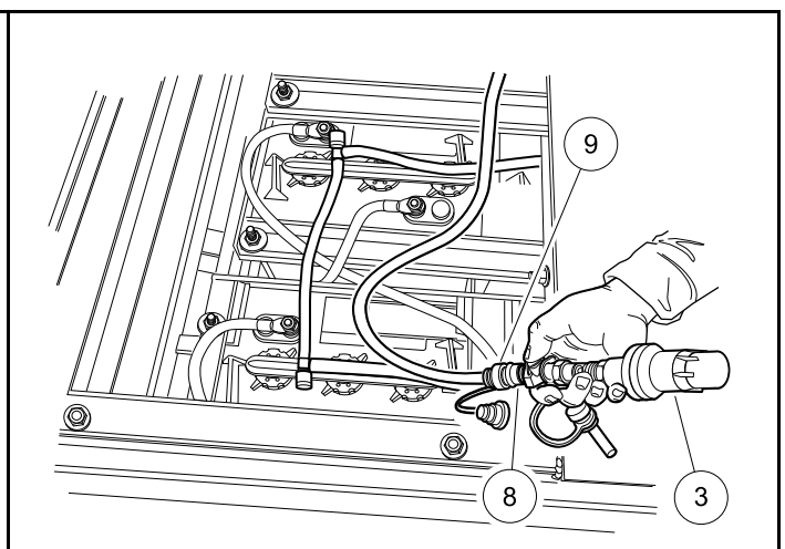
Figure 28 Connecting Hose-end Assembly to Battery Fill Connector
