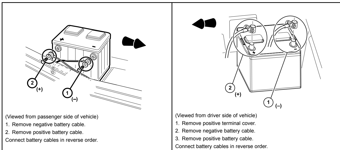
Figure 4 Top-Post Battery- Battery Cable Removal-Gasoline Vehicles
