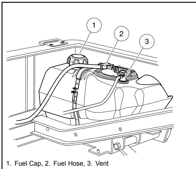
Figure 39 Fuel Tank
