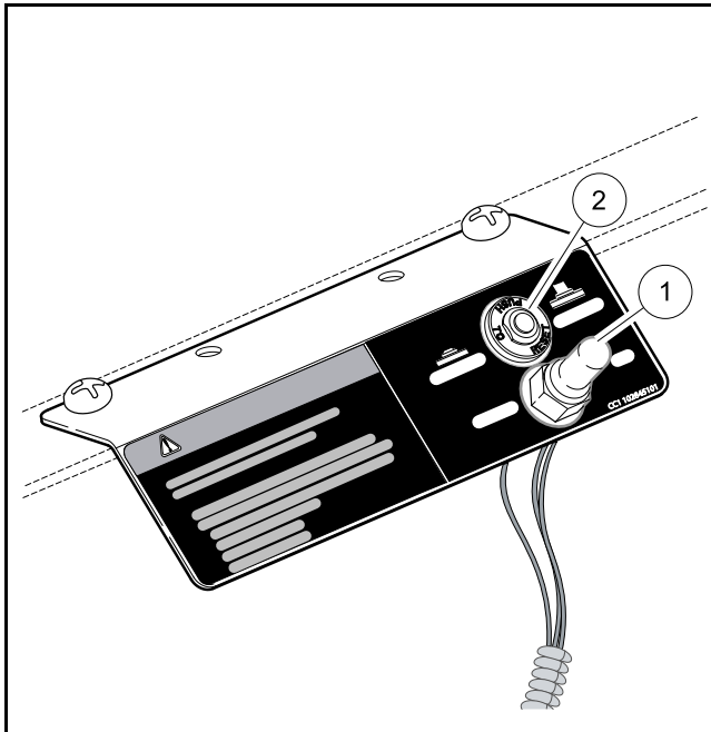
Figure 16 Tow/Run Switch
