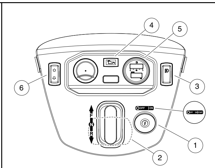
Figure 11 Instrument Panel – Gasoline Vehicles
