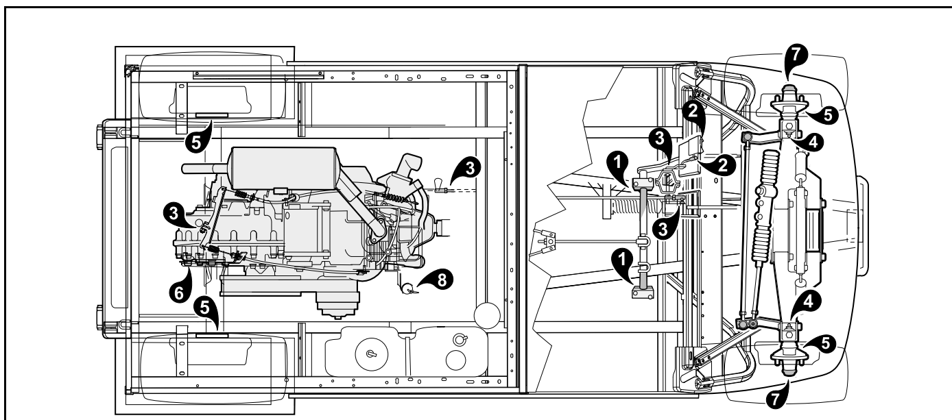
2823 Figure 22 Lubrication Points – Gasoline Vehicles
