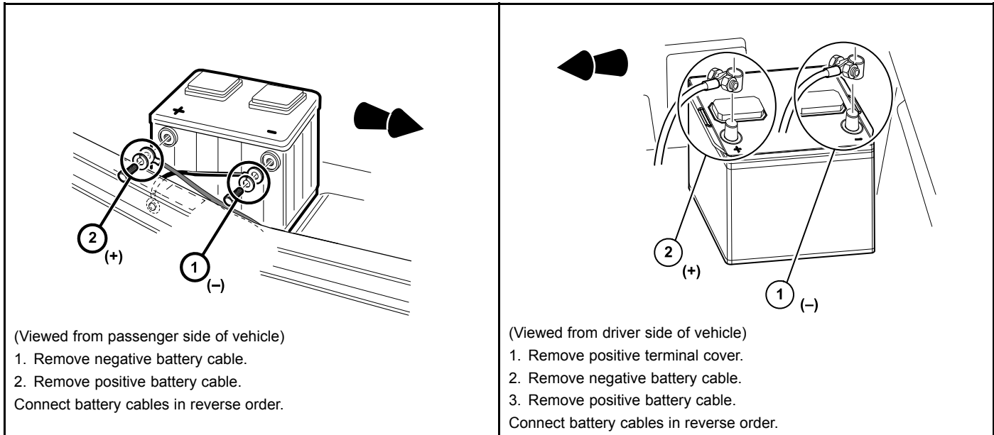
Figure 6 Top-Post Battery- Battery Cable Removal-Gasoline Vehicles
